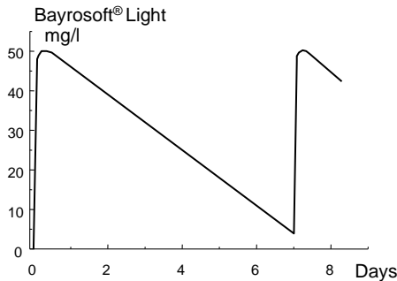
Automatic dosing at 24 °C (Trend of the Bayrosoft® Light concentration over one week)
